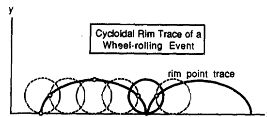
Figure 10.7. Trace of the rim point of a rolling wheel.
