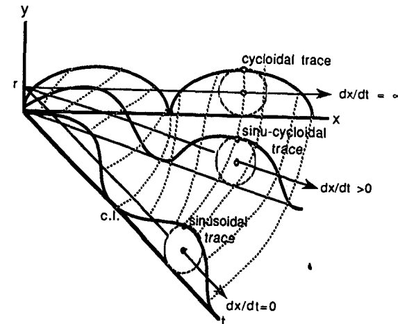
Figure 10.9. Dynamical traces of a wheel rolling event. Here, r is the radius of rotation and c.l. is the circumferential length. The information specifying the TIs for such events clearly has an intrinsic scale.
