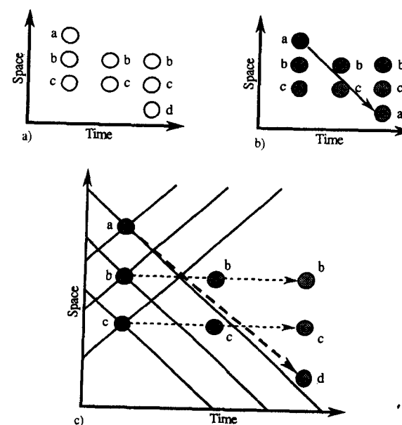
Figure 10.22. The Ternus effect II. The timing has been changed so that an apparent motion is seen between the dots on the ends even though the two middle dots are not seen to move.
