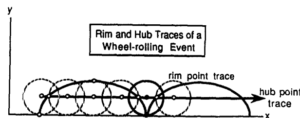
Figure 10.8. Hub point and rim point traces of a rolling wheel.
