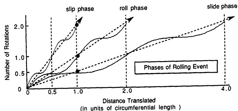
Figure 10.12. Three phases of a rolling event arise from an object rotating with different degrees of frictional contact with a given surface. Slip phase: with some slipping the wheel rotates more than once for each circumferential length over which it translates. Roll phase: with perfect traction the wheel rotates exactly once for each circumferential length over which it translates. Slide phase: with the application of some outside pulling force the wheel rotates less than once for each circumferential length over which it translates
