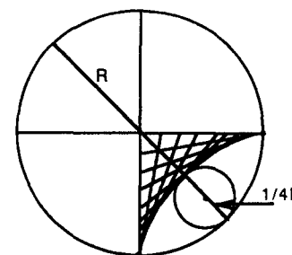
Figure 10.11. A chord distribution geometry. An integral geometry based on chord-sets rather than point-sets provides one way of smoothing out discontinuities (Moore, 1971, 1972) (see text for details).
