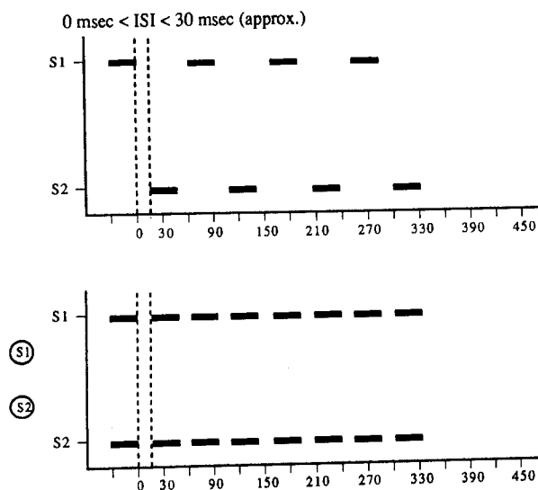
Figure 10.17. Apparent motion (phase 5): at an ISI of less than approx. 30 ms two simultaneous events with no motion of any kind are seen.
