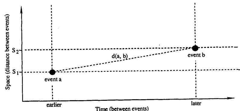
Figure 10.19. Galilean event diagram.
