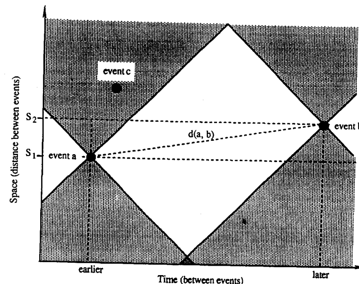
Figure 10.20. Restricted Minkowski-like event diagrams. The intervals between events in this geometry are restricted. The slopes of the lines define forward (anticipatory) and backward (hereditary) cones within which events may causally interact (light color). The forward causal cone is shown here as defined from the perspective of event a with respect to event b . There are also null cones (dark color) representing regions in which no causal action can take place between events. For instance, since event c lies in the null cone of event a , they cannot causally interact. Rather, they are effectively simultaneous. Worldlines may not cross unless there is a merger of object identity. Objects with mass do not mechanically interact this way since one palpable volume must displace another and cannot occupy the same place at the same time.
