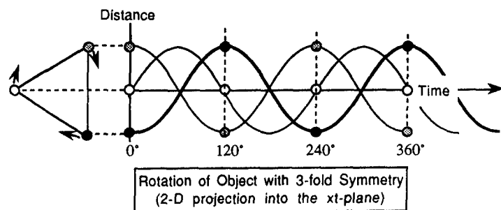
Figure 10.3. The 3-fold symmetry of the trace of a rotating triangle (2-D projection into the xt plane).
