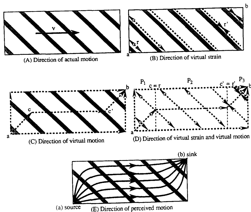
Figure 10.10. Perception of apparent direction.
