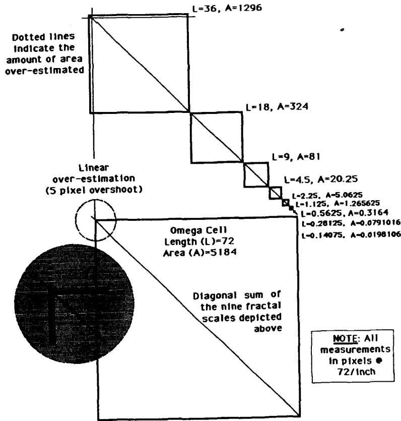
Fig. 14. Alpha limits on precision of fractal scaling.
