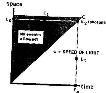
Fig. 3. Two-dimensional section of a four-dimensional spacetime.
