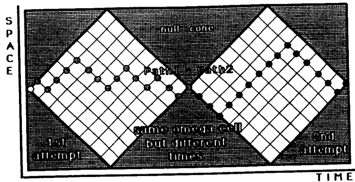
Fig. 10. Omega cells define conservative fields.
