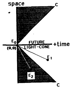
Fig. 4. The future light-cone.
