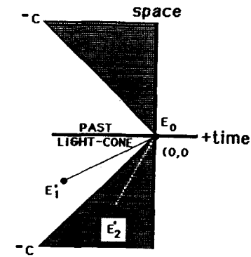
Fig. 5. The past light-cone.
